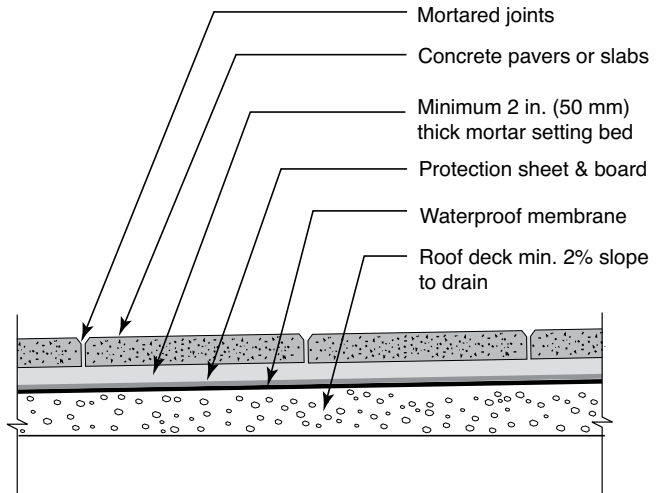
Figure 10. Mortar bed under paving units
