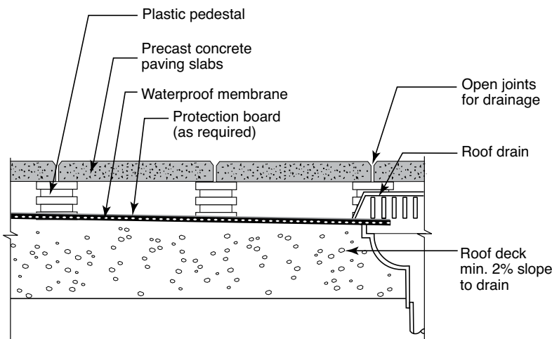
Figure 5. Paving slabs on pedestals
