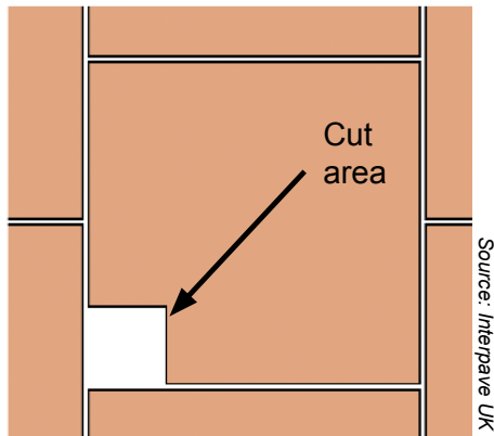
Figure 24. Cut areas less than 25% of the slab area generally do not require additional cuts on the paving slab to reduce the risk of cracking.
