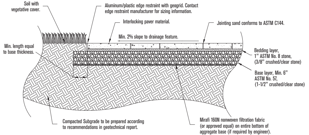
Typical cross-section of open-graded paver base construction/installation.
