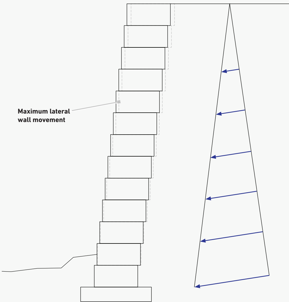
Figure 14.4 | Wall Section
